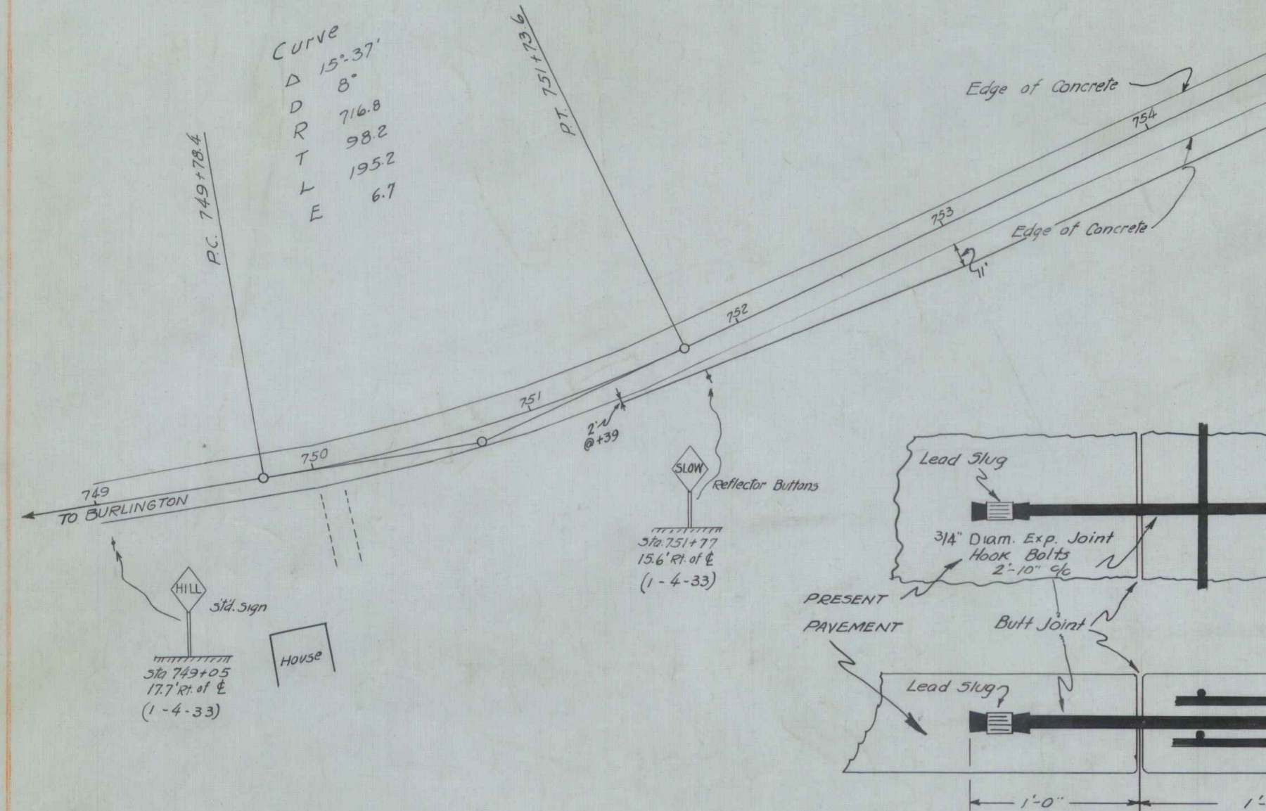
SKETCH SHOWING EXPANSION HOW NEW PAVEMENT TO PRESENT PAVEMENT THE NEW PAVEMENT IS LESS THAN 10
